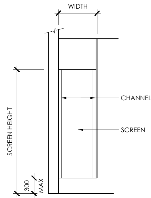
4 TYPICAL SCREEN ELEVATION SCALE 1:30
