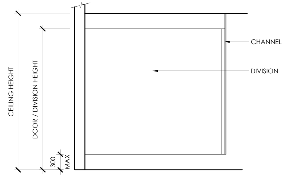
3 TYPICAL TOILET DIVISION ELEVATION SCALE 1:30
