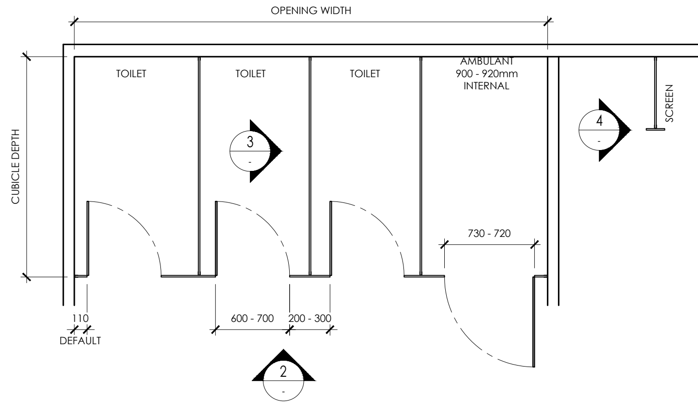
1 TYPICAL TOILET ARRANGEMENT LAYOUT SCALE 1:30
